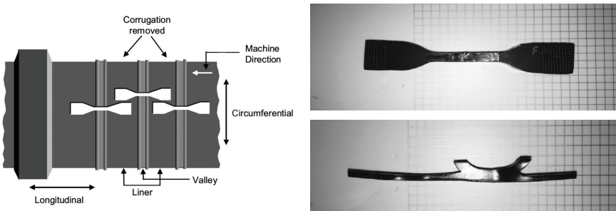
Figure 8.4: Illustration of junction specimen sampling procedure and images of specimens
