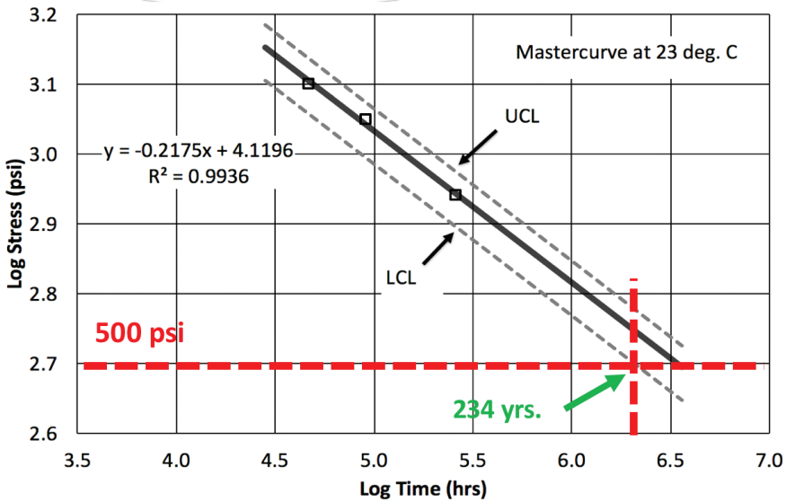
Figure 8.8: Service life projection for 30-in. (750 mm) diameter pipe manufactured with 49% post-consumer recycled materials based on applying Popelar Shift Factors to UCLS test results at three independent test conditions (80 deg. C / 650 psi, 70 deg. C, 650 psi, and 80 deg. C, 450 psi)
