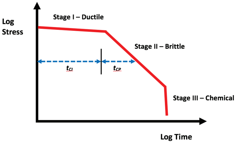
Figure 8.7: The service life of pipes manufactured with recycled materials relative to Stage II cracking is a function of the time for cracks to initiate, t_{ci} , plus the time for them to propagate, t_{cp}
